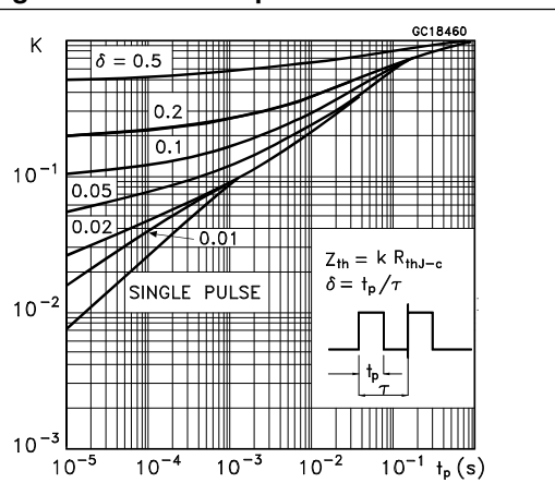
Figure 7. Thermal impedance for TO-247
