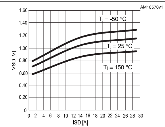
Figure 17. Source-drain diode forward vs temperature
