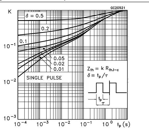
Figure 3. Thermal impedance for TO-220FP
